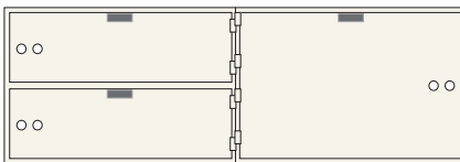
AXL-3-10 (Wt. 140 lbs.) 2 openings ea. 5" x 16" 1 openings ea. 10" x 16"
