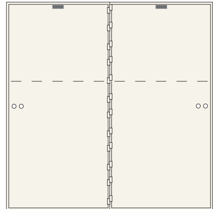
AXL-2-33 (Wt. 280 lbs.) 2 openings ea. 33" x 16"
