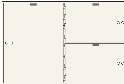
AXL-3-22 (Wt. 195 lbs.) 1 opening 22" x 16" 2 openings ea. 10" x 16"
